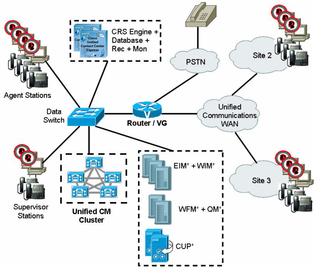
Figure 4-2 depicts the deployment when integrating Unified CCX with Cisco Unified Communications Manager Express (Cisco Unified CME).
