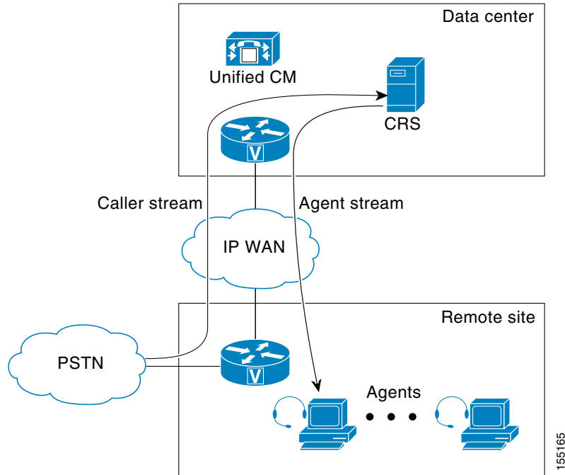
Figure 7-3 Call from PSTN to Cisco Unified CCX Server to Agent
